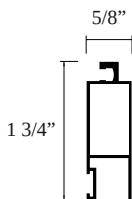
Vertical Mosquitero 26534
